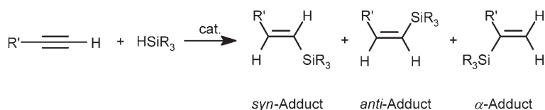
Scheme 1. Hydrosilylation of terminal alkynes.
